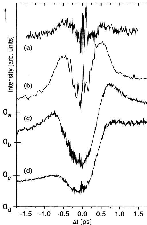
FIG. 2. NeNePo spectra of the silver trimer taken with wavelengths of (a) \lambda = 390 nm, (b) \lambda = 400 nm, (c) \lambda = 415 nm, (d) \lambda = 420 nm. Note that each curve, (a) through (d), has its own axis of zero signal, and that the time-independent background increases steadily with decreasing wavelength. The fine structure around \Delta t = 0 is, as in Fig. 1, due to interference of pump and probe pulses.
